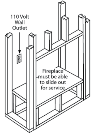
(B) Raised Framing
